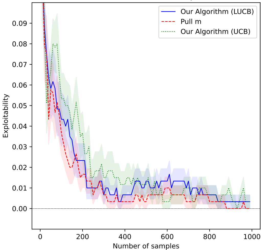
Kuhn Poker, Variations, Player o
